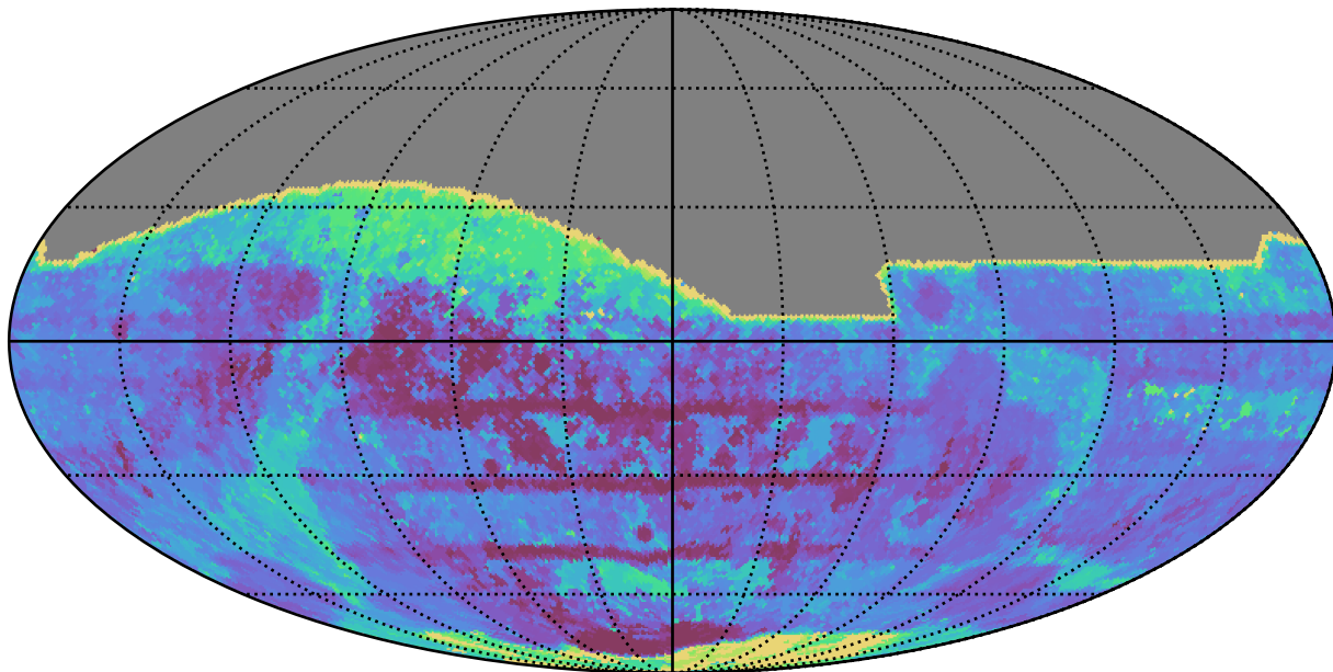
weather_cloudso8v3.4_10yrs All sky all bands: Max Inter-Night Gap
