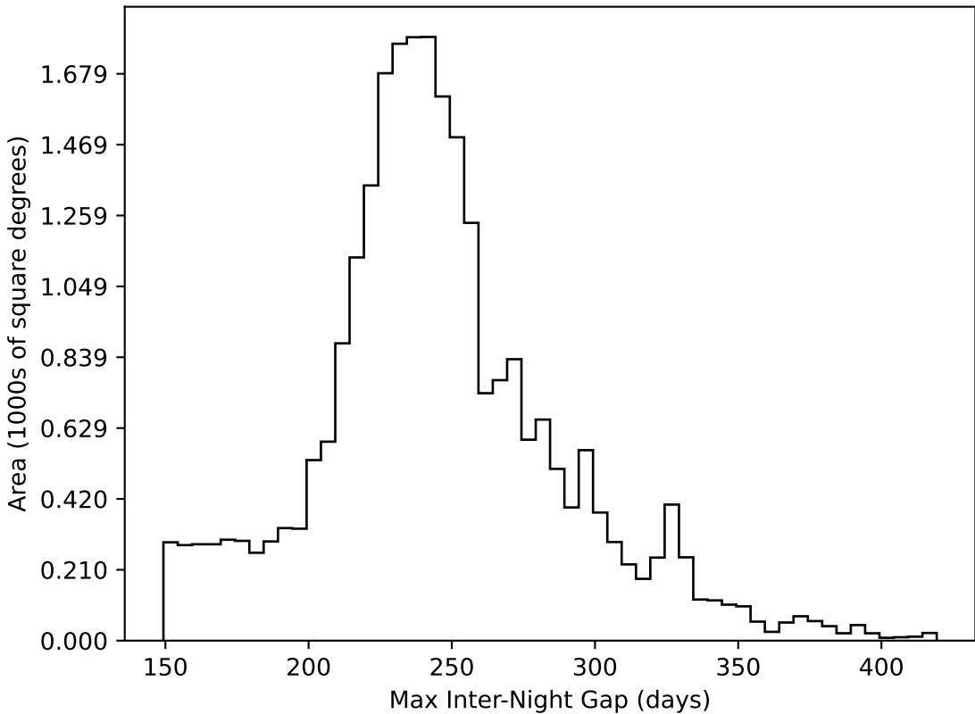
weather_cloudso8v3.4_10yrs All sky all bands: Max Inter-Night Gap
