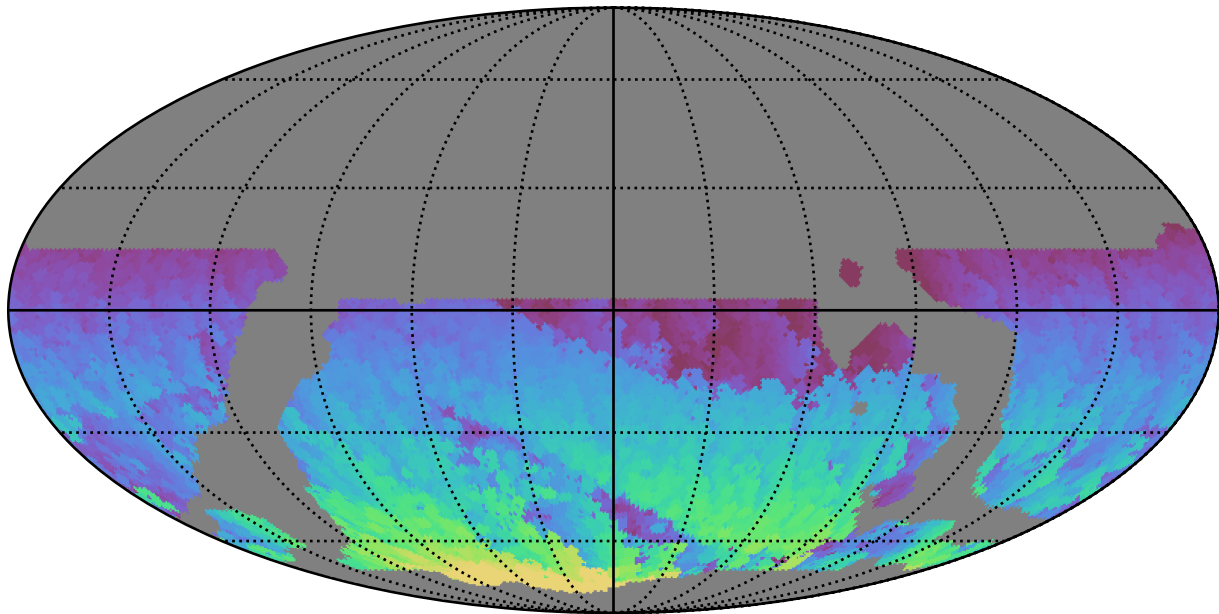
weather_cloudso8v3.4_10yrs WFD z band: Max HA
