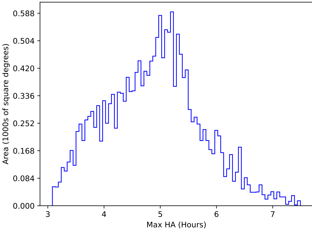
weather_cloudso8v3.4_10yrs WFD z band: Max HA
