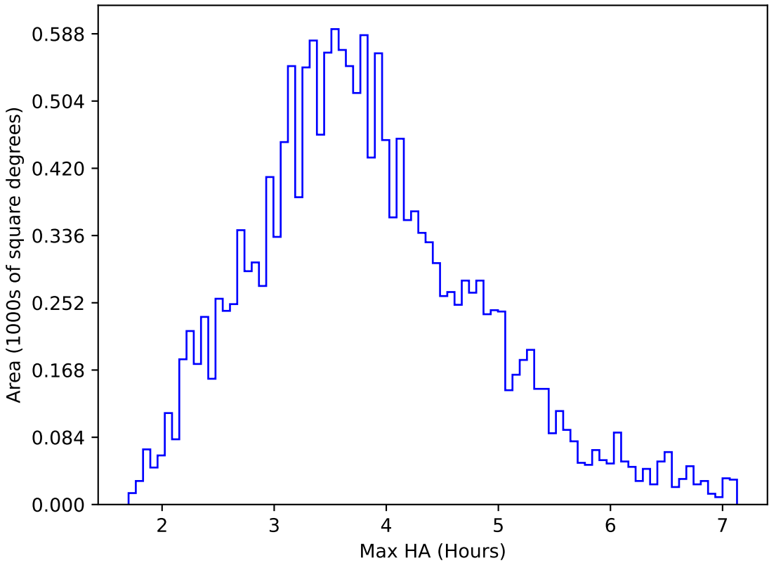
weather_cloudso8v3.4_10yrs WFD u band: Max HA
