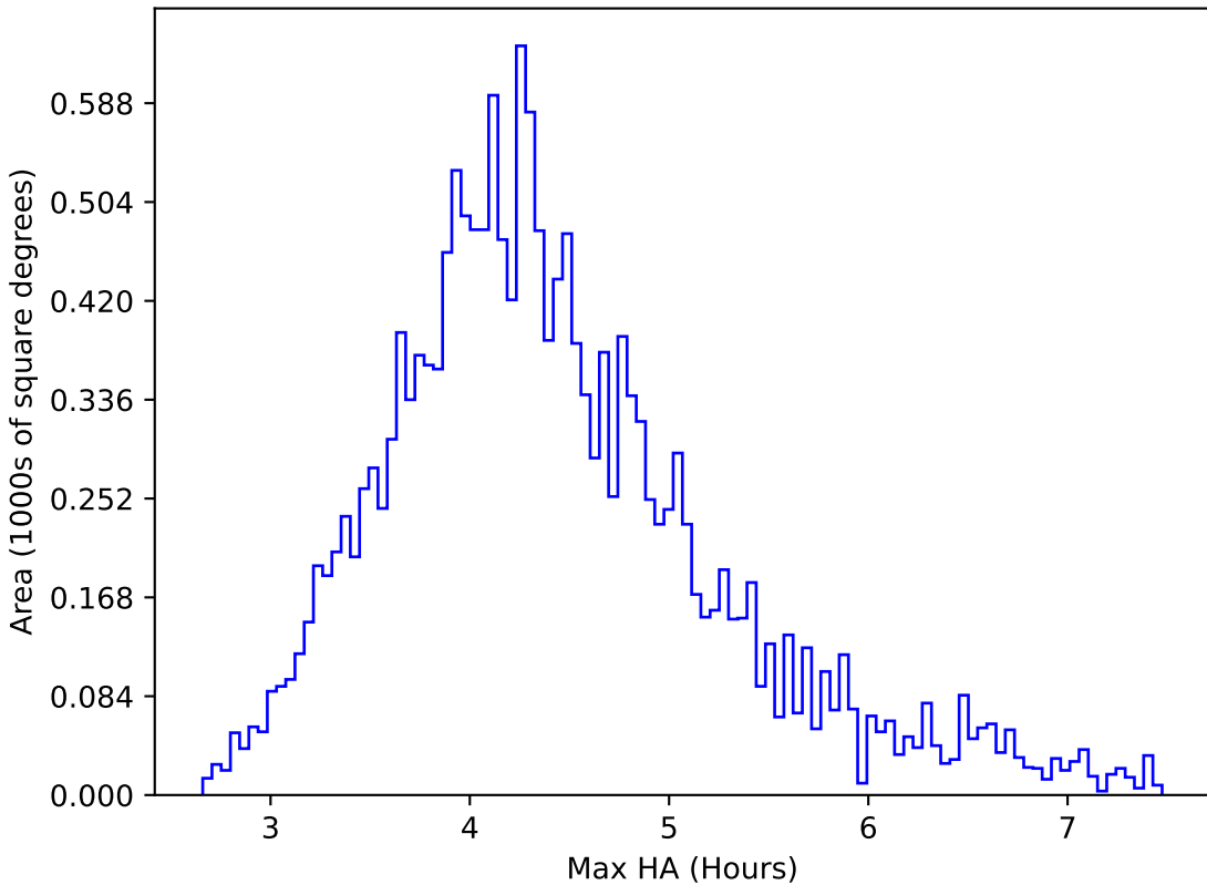
weather_cloudso8v3.4_10yrs WFD r band: Max HA
