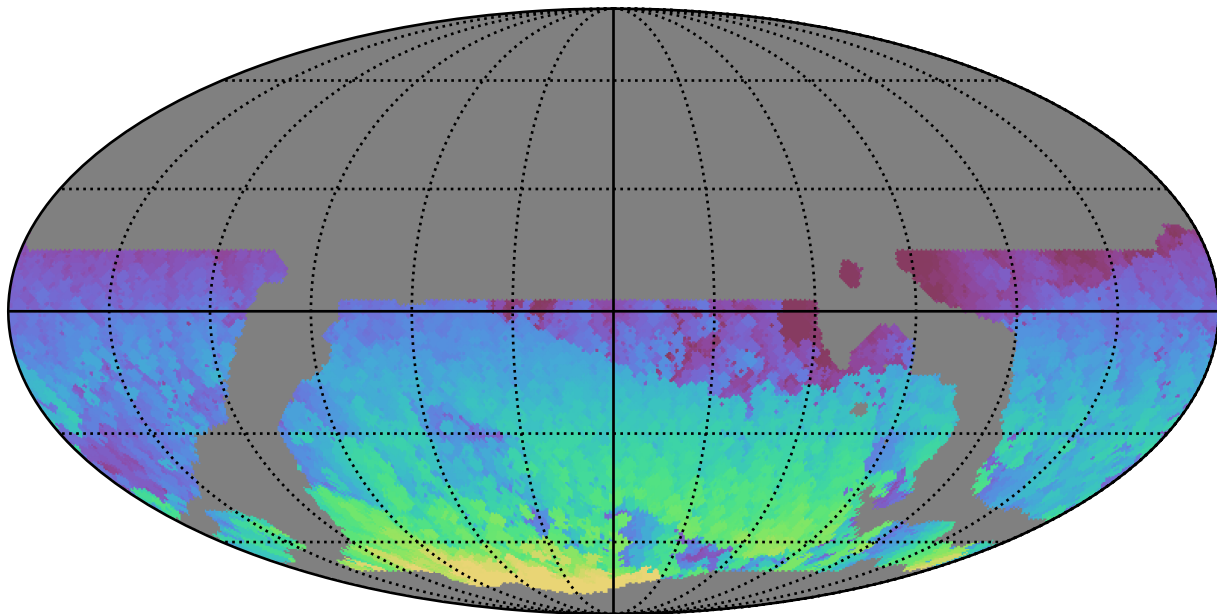
weather_cloudso8v3.4_10yrs WFD i band: Max HA
