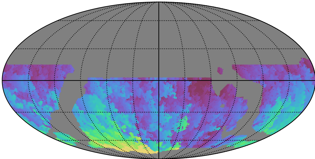
weather_cloudso8v3.4_10yrs WFD g band: Max HA
