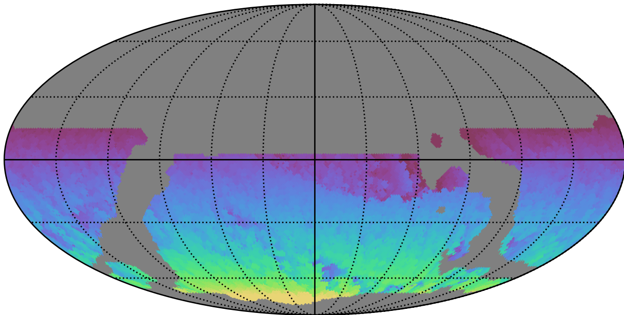
weather_cloudso8v3.4_10yrs WFD all bands: Max HA
