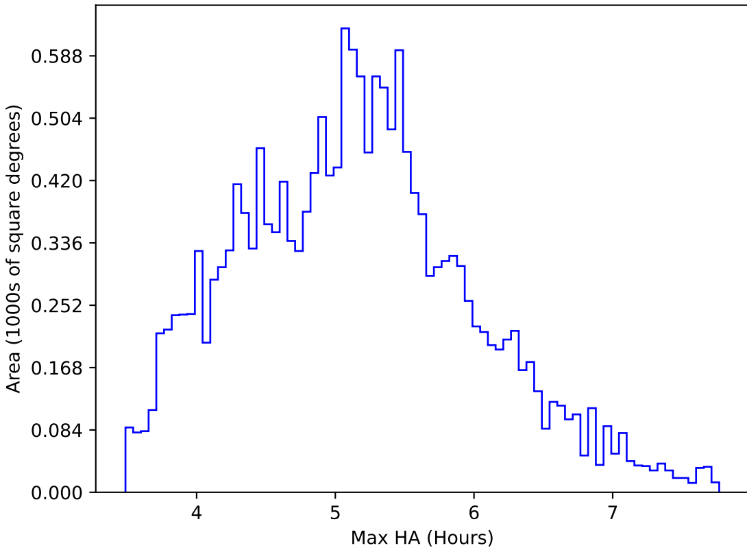
weather_cloudso8v3.4_10yrs WFD all bands: Max HA
