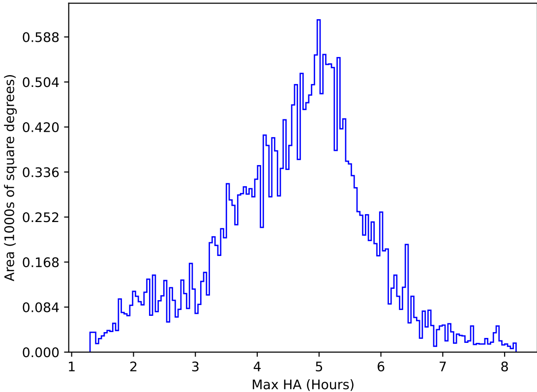
weather_cloudso8v3.4_10yrs All sky z band: Max HA
