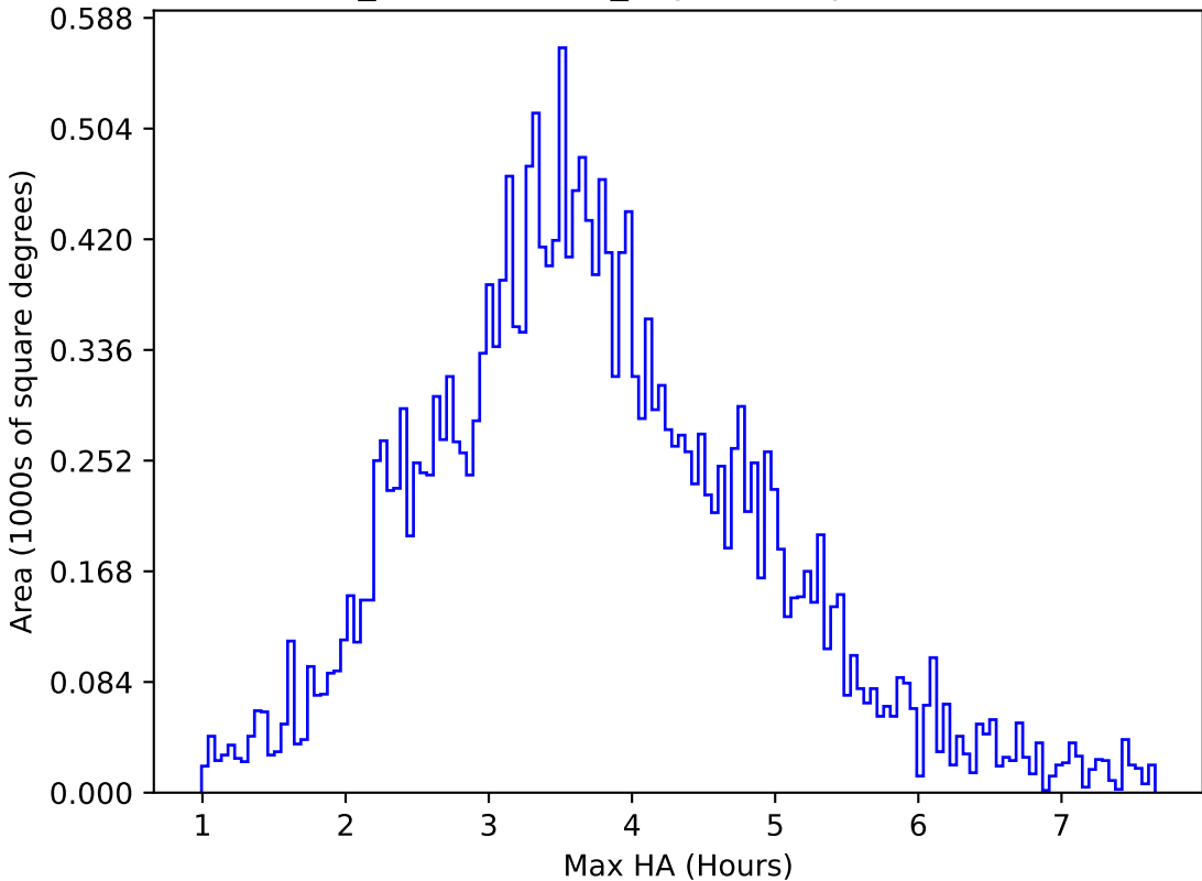
weather_cloudso8v3.4_10yrs All sky u band: Max HA
