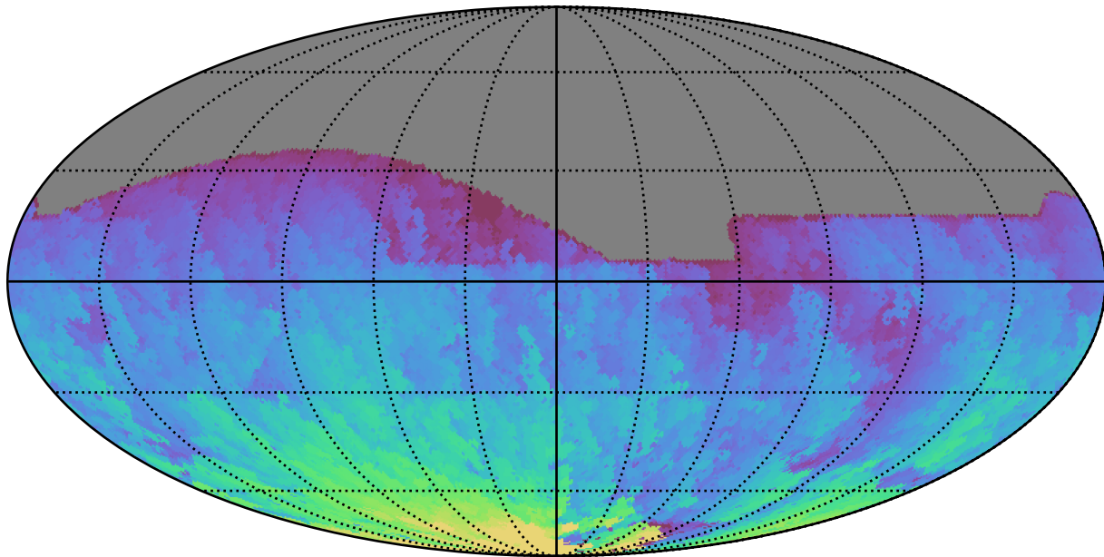
weather_cloudso8v3.4_10yrs All sky r band: Max HA
