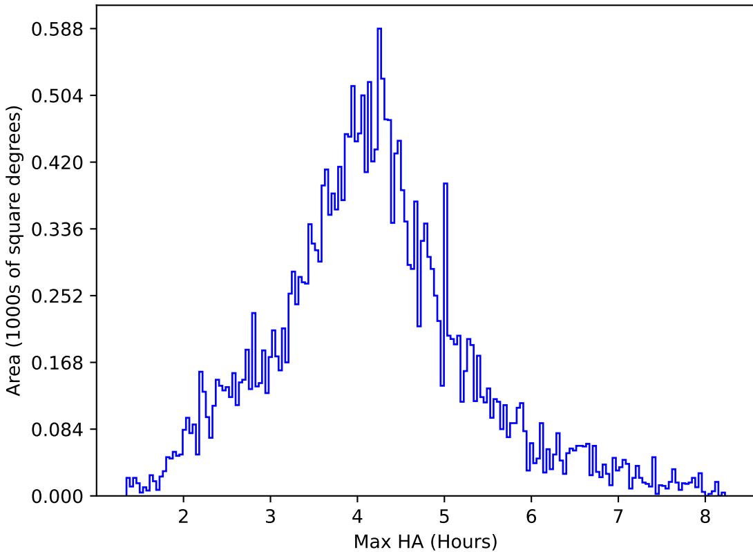
weather_cloudso8v3.4_10yrs All sky r band: Max HA
