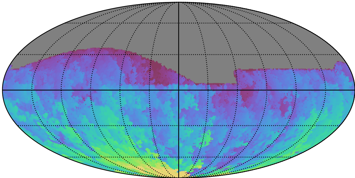
weather_cloudso8v3.4_10yrs All sky g band: Max HA
