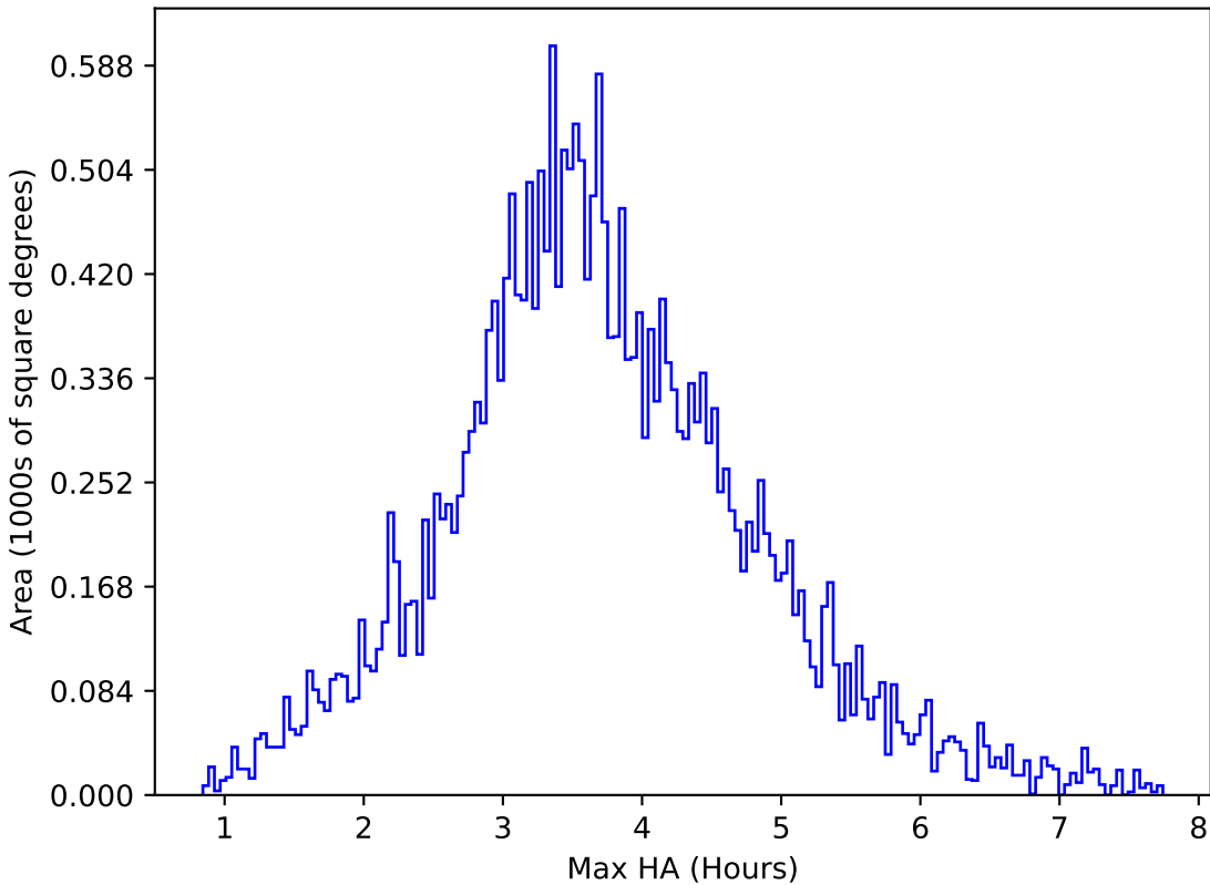
weather_cloudso8v3.4_10yrs All sky g band: Max HA
