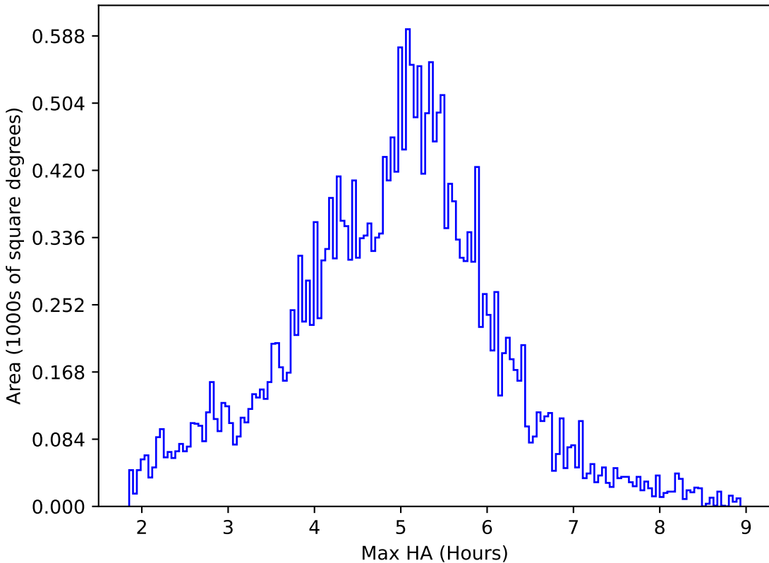
weather_cloudso8v3.4_10yrs All sky all bands: Max HA
