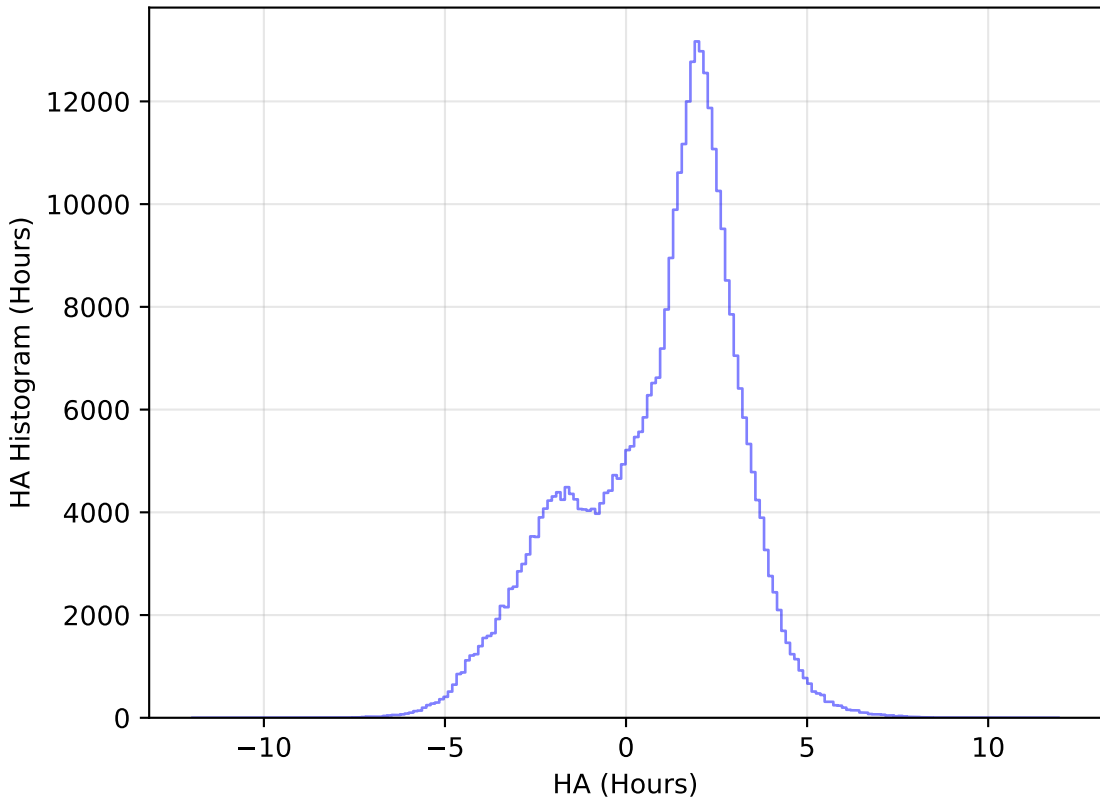
weather_cloudso8v3.4_10yrs WFD y band: HA Histogram
