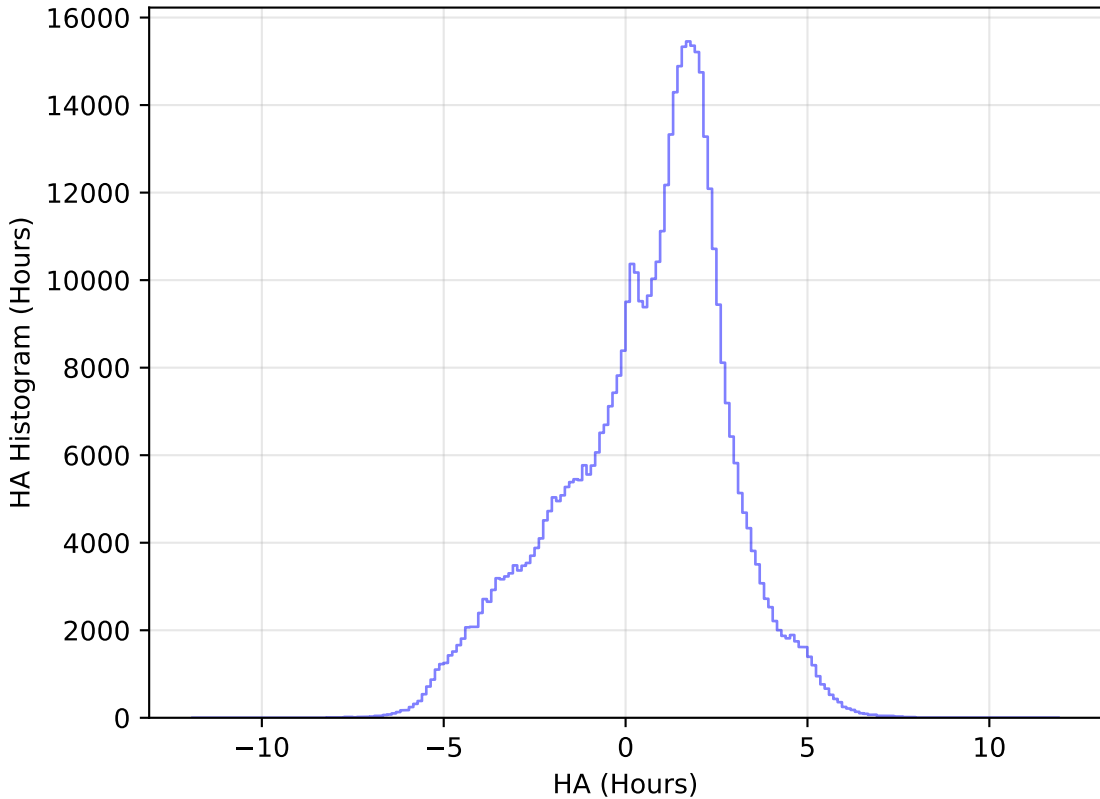
weather_cloudso8v3.4_10yrs WFD i band: HA Histogram
