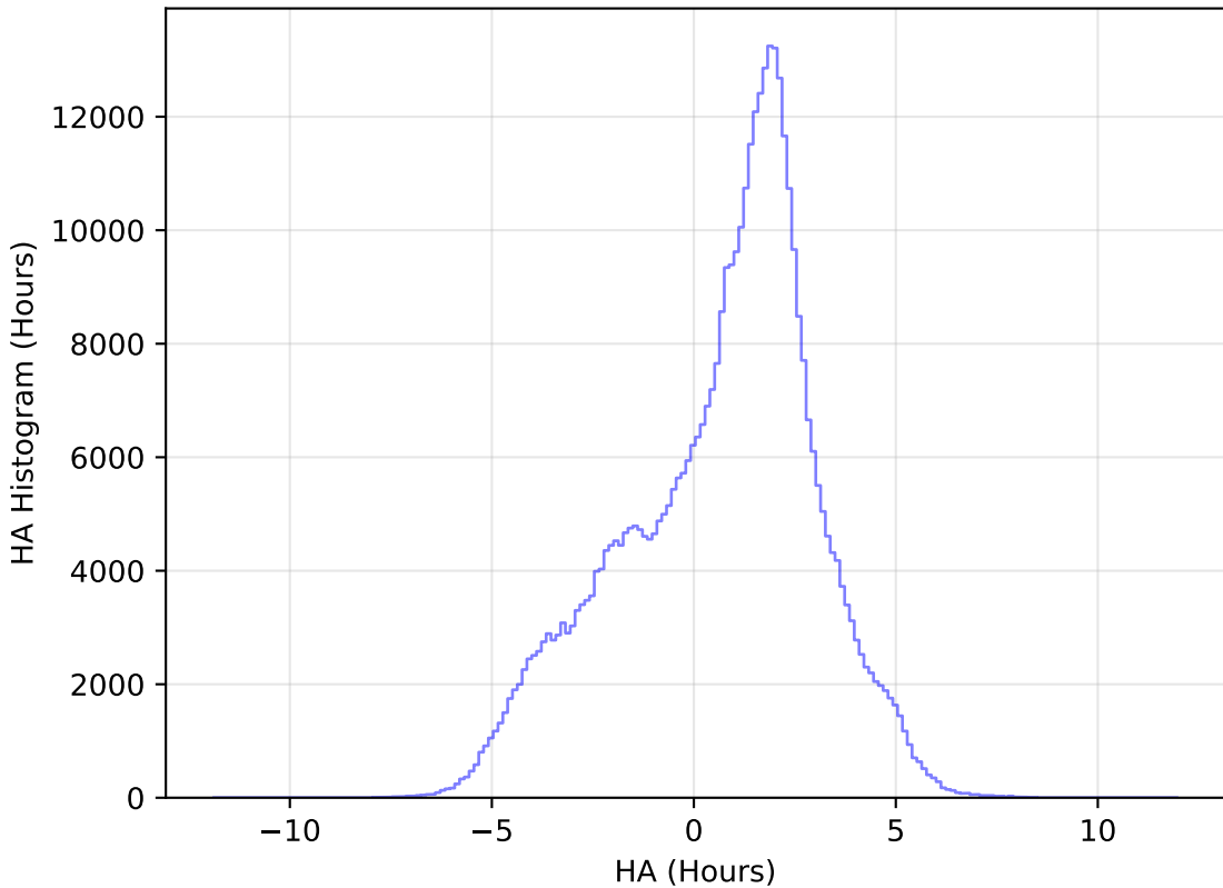
weather_cloudso8v3.4_10yrs All sky z band: HA Histogram
