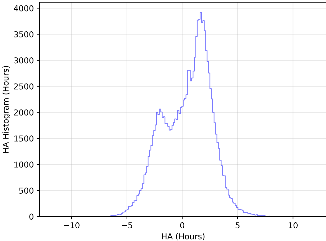
weather_cloudso8v3.4_10yrs All sky u band: HA Histogram
