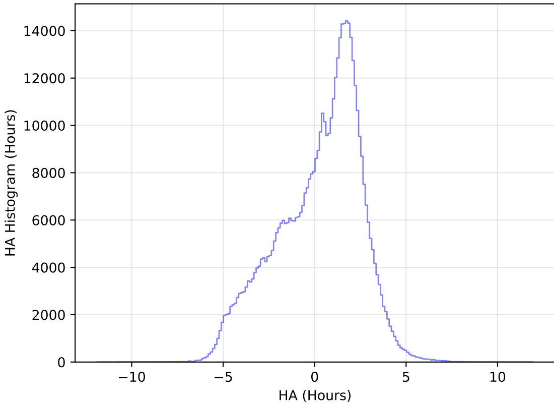
weather_cloudso8v3.4_10yrs All sky r band: HA Histogram
