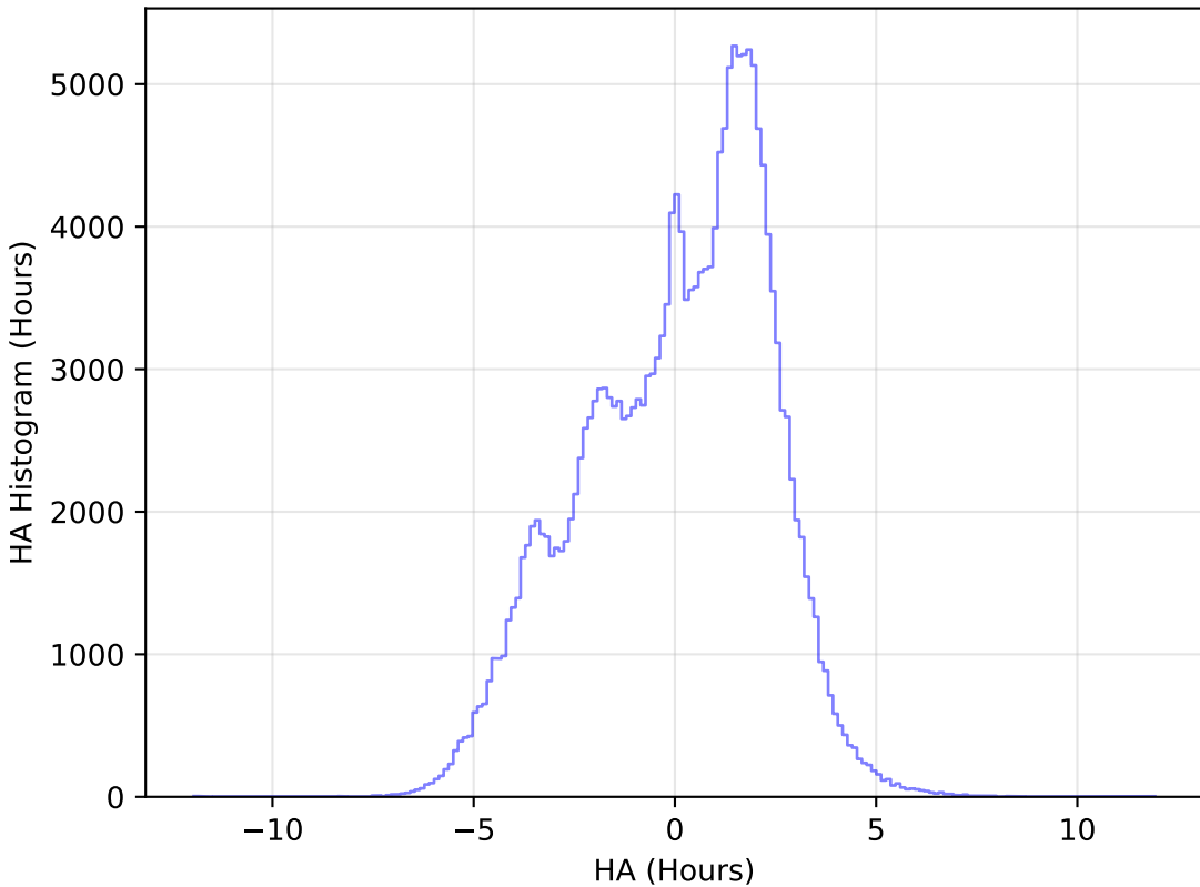
weather_cloudso8v3.4_10yrs All sky g band: HA Histogram
