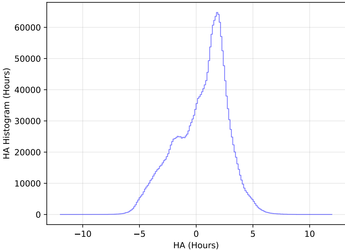
weather_cloudso8v3.4_10yrs All sky all bands: HA Histogram
