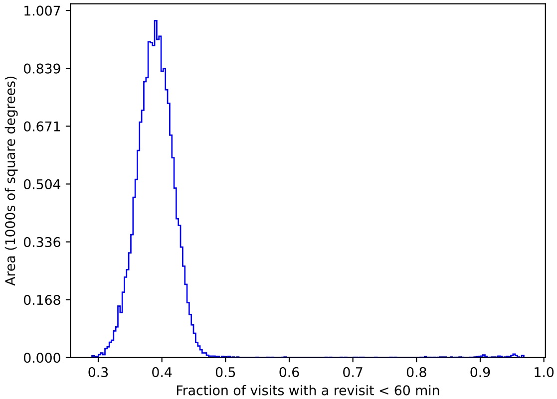
weather_cloudso8v3.4_10yrs gri WFD: Fraction of visits with a revisit < 60 min
