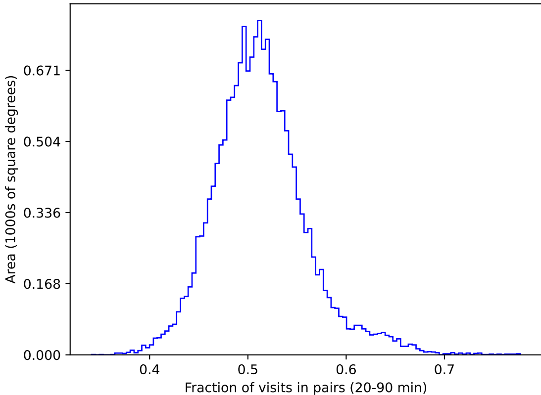
weather_cloudso8v3.4_10yrs gri WFD: Fraction of visits in pairs (20-90 min)
