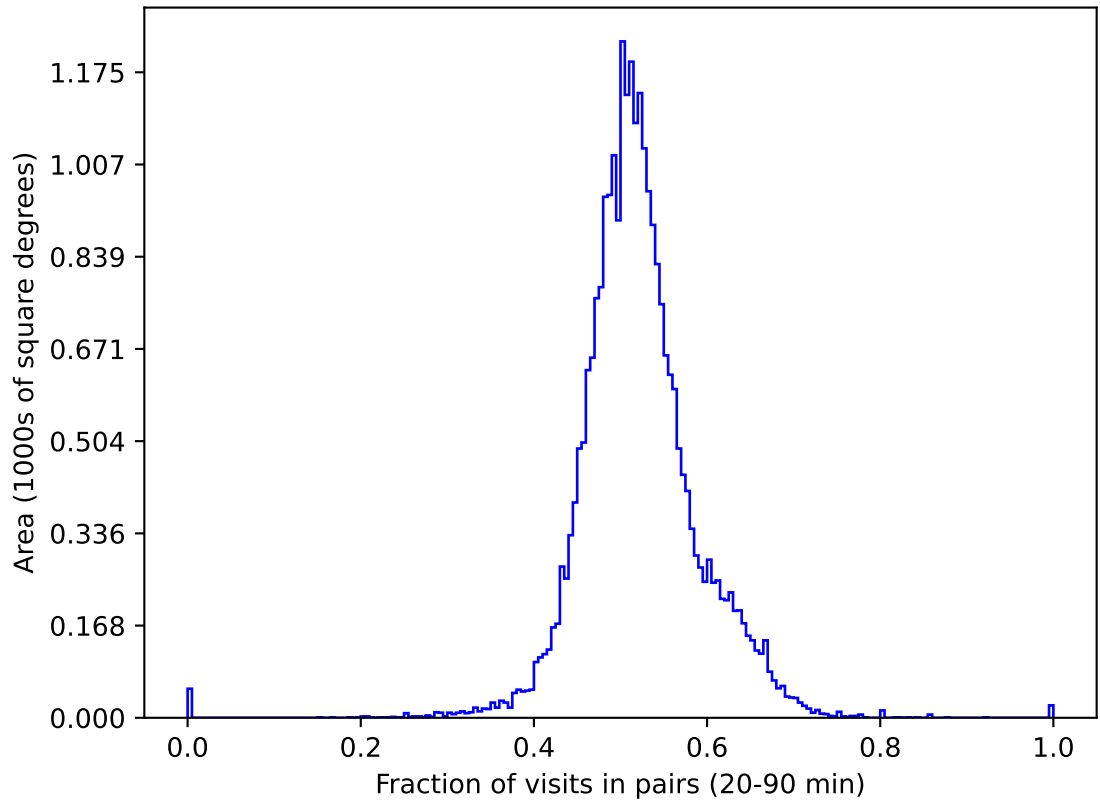
weather_cloudso8v3.4_10yrs gri All sky: Fraction of visits in pairs (20-90 min)
