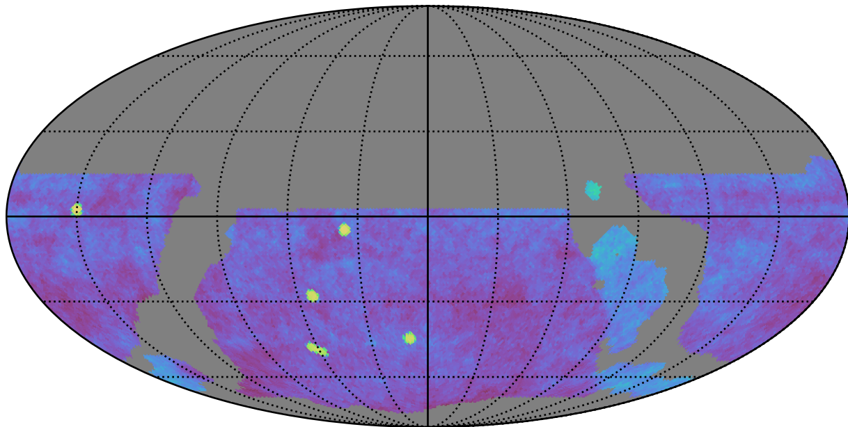
weather_cloudso8v3.4_10yrs gri WFD: Fraction of visits in pairs (10-60 min)
