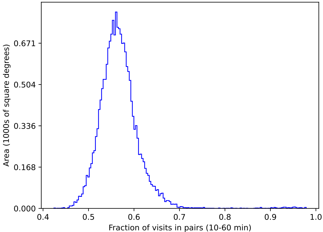
weather_cloudso8v3.4_10yrs gri WFD: Fraction of visits in pairs (10-60 min)
