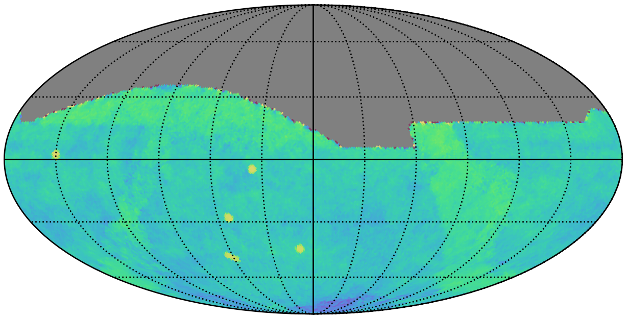
weather_cloudso8v3.4_10yrs gri All sky: Fraction of visits in pairs (10-60 min)
