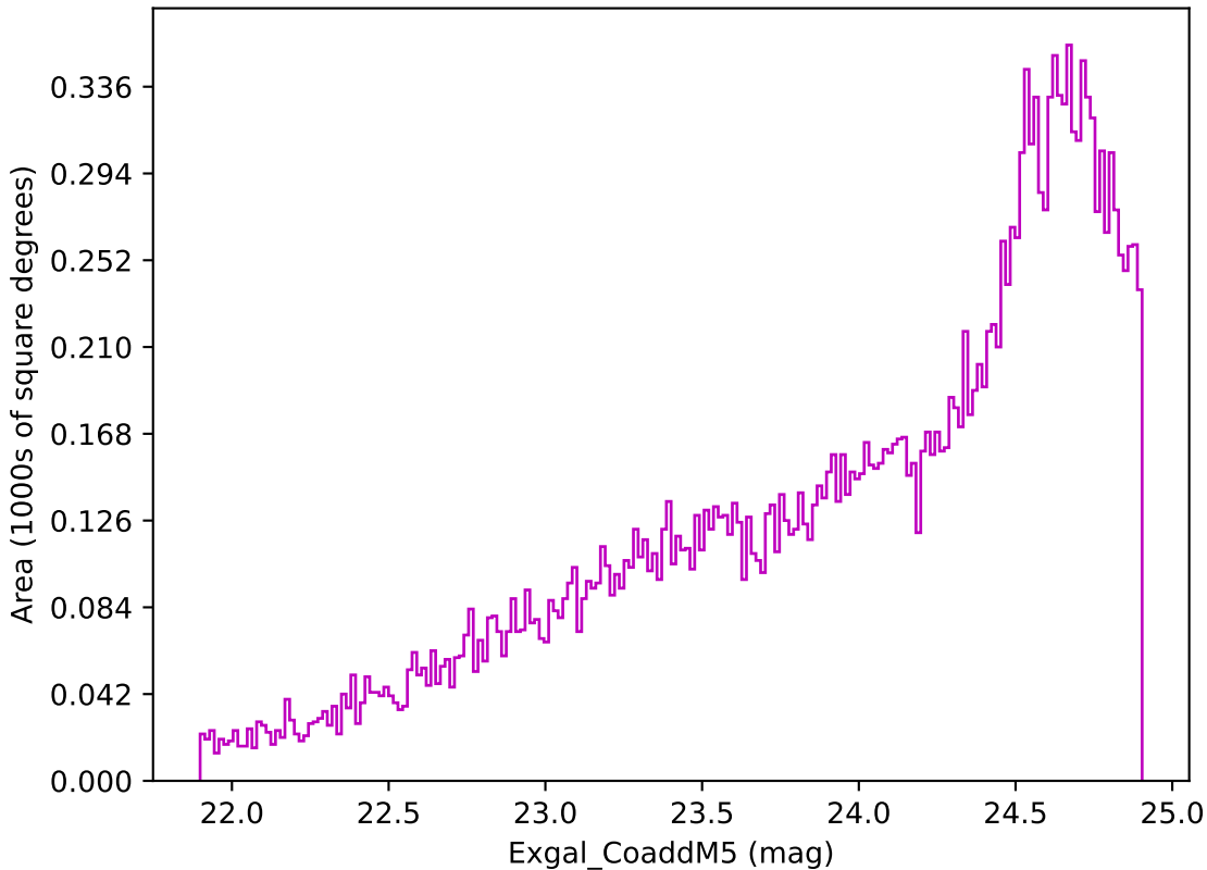
weather_cloudso8v3.4_10yrs Yr 3-4 z band: Exgal_CoaddM5
