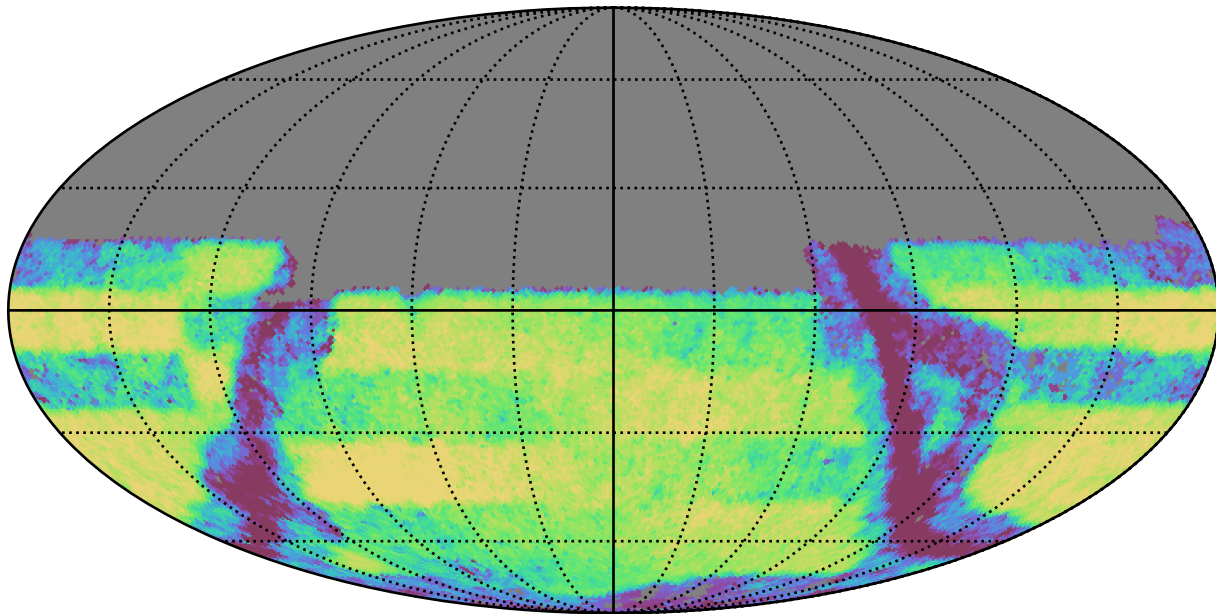
weather_cloudso8v3.4_10yrs Yr 3-4 y band: Exgal_CoaddM5
