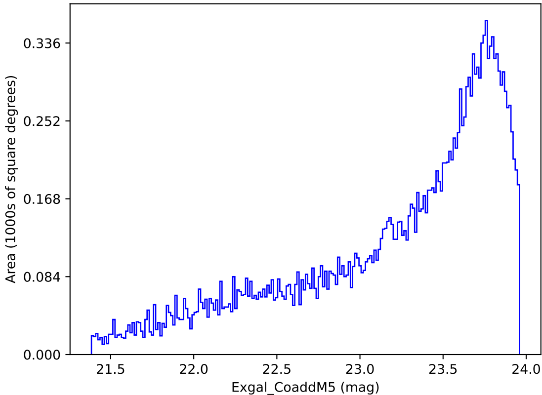
weather_cloudso8v3.4_10yrs Yr 3-4 y band: Exgal_CoaddM5
