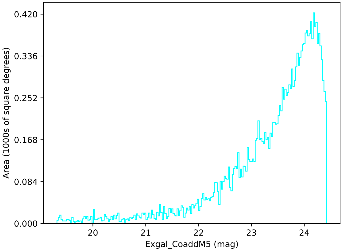
weather_cloudso8v3.4_10yrs Yr 3-4 u band: Exgal_CoaddM5
