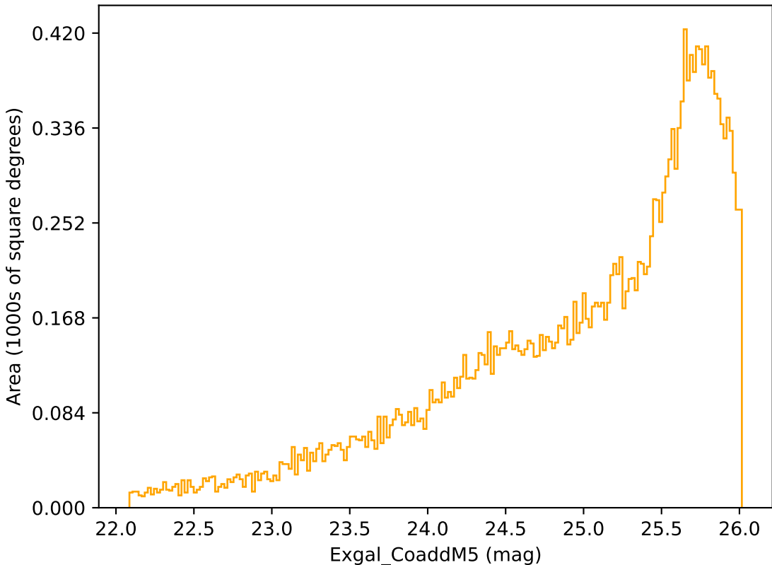
weather_cloudso8v3.4_10yrs Yr 3-4 r band: Exgal_CoaddM5
