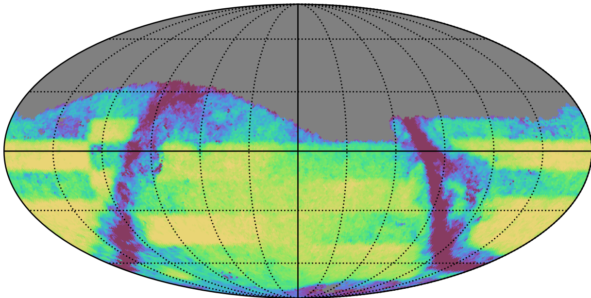
weather_cloudso8v3.4_10yrs Yr 3-4 i band: Exgal_CoaddM5
