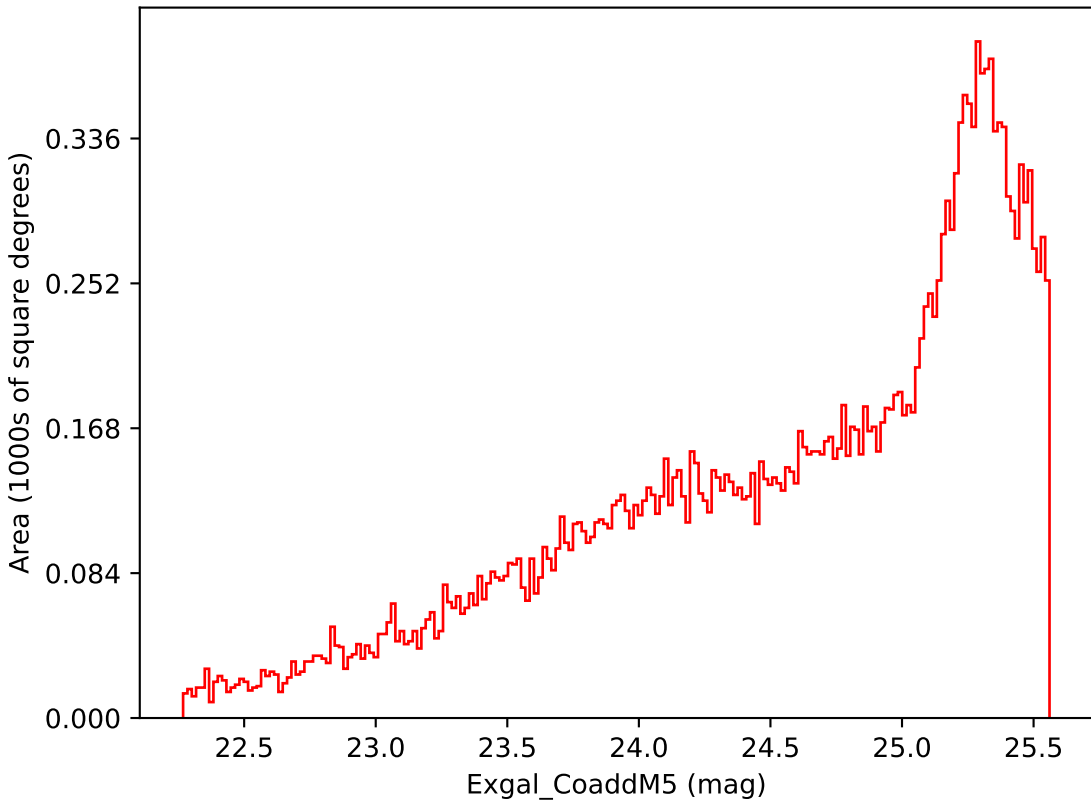
weather_cloudso8v3.4_10yrs Yr 3-4 i band: Exgal_CoaddM5
