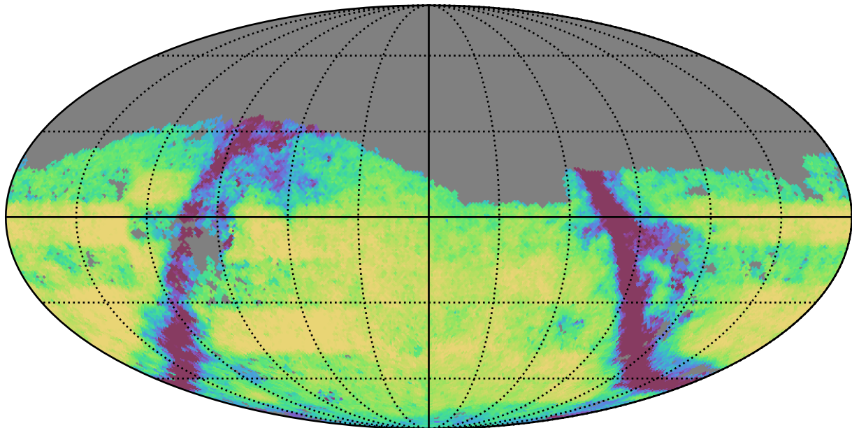
weather_cloudso8v3.4_10yrs Yr 3-4 g band: Exgal_CoaddM5
