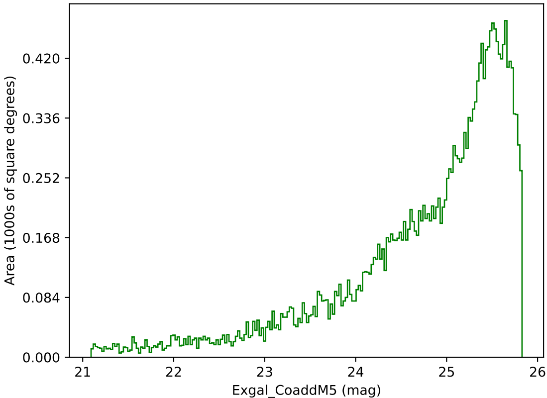
weather_cloudso8v3.4_10yrs Yr 3-4 g band: Exgal_CoaddM5
