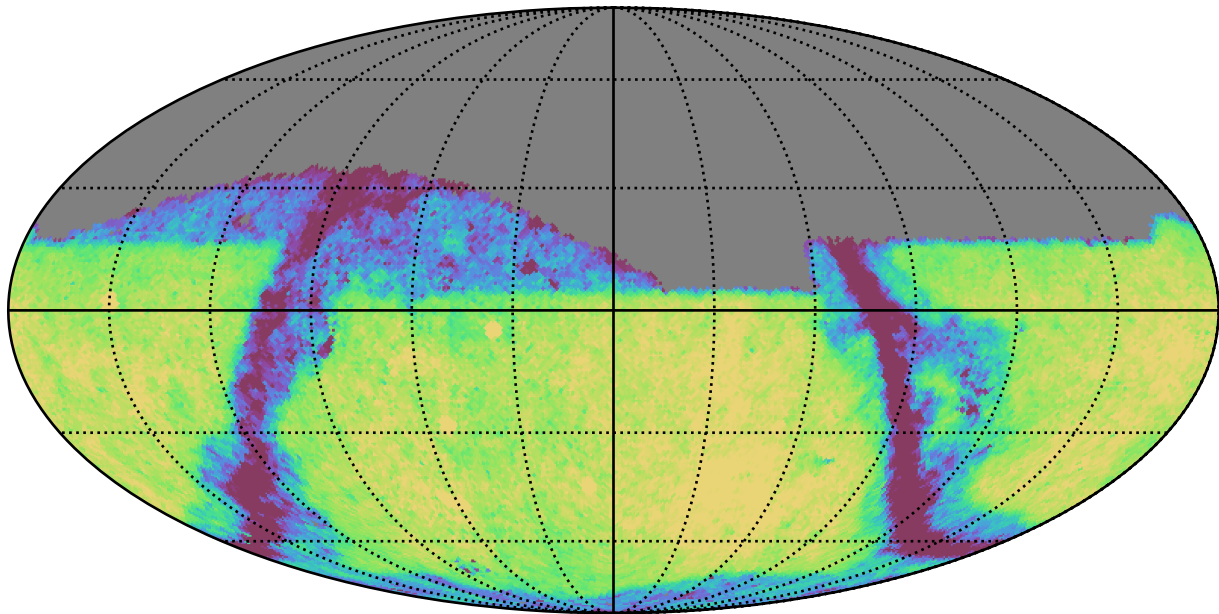
weather_cloudso8v3.4_10yrs Yr 1 z band: Exgal_CoaddM5
