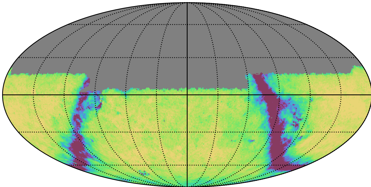
weather_cloudso8v3.4_10yrs Yr 1 u band: Exgal_CoaddM5
