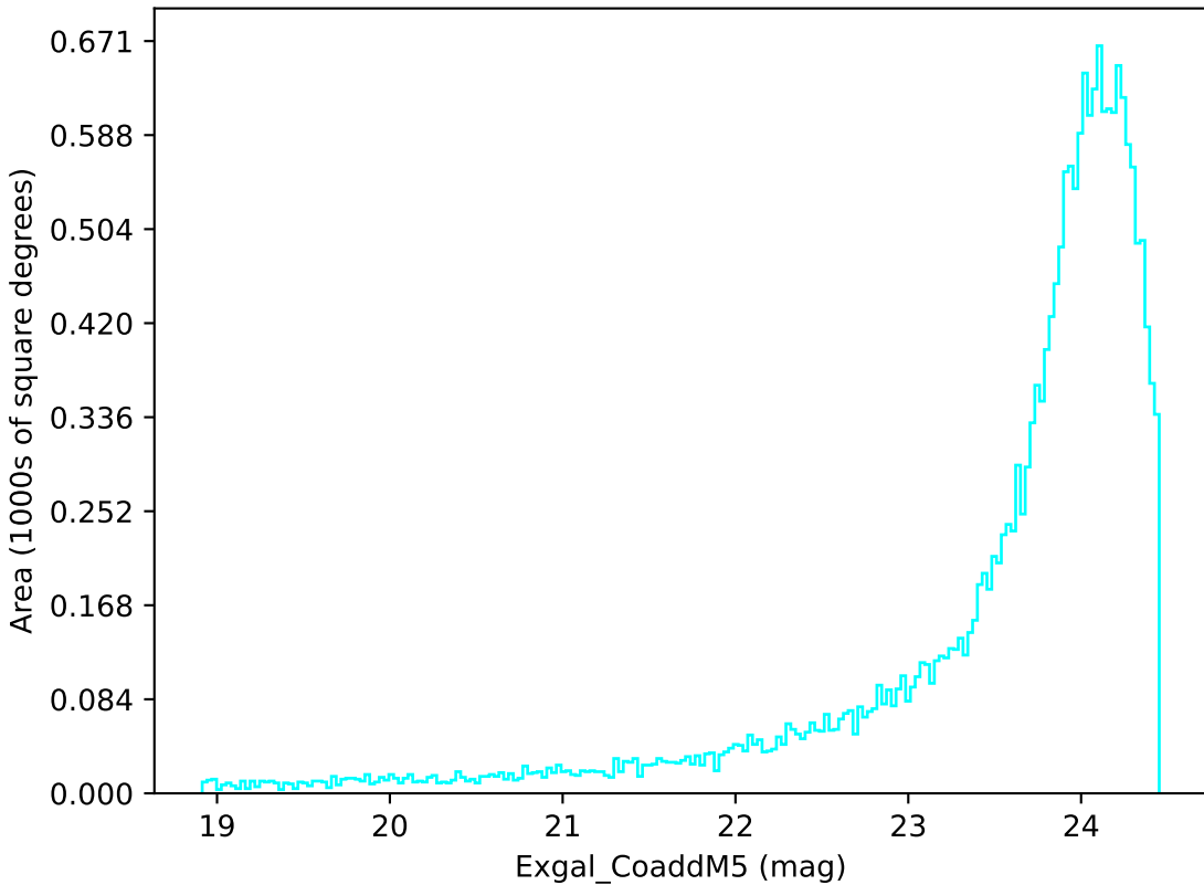
weather_cloudso8v3.4_10yrs Yr 1 u band: Exgal_CoaddM5
