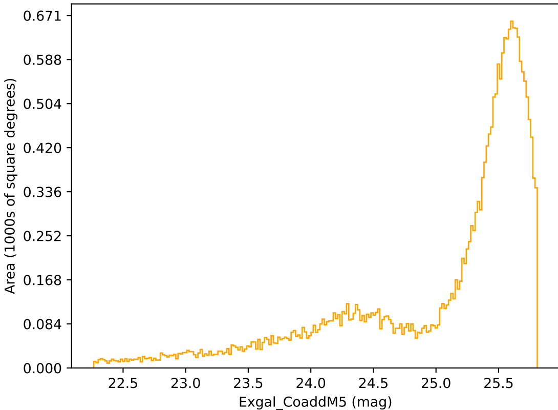
weather_cloudso8v3.4_10yrs Yr 1 r band: Exgal_CoaddM5
