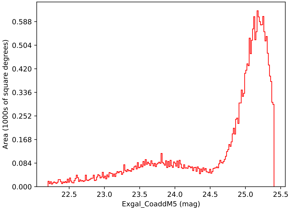
weather_cloudso8v3.4_10yrs Yr 1 i band: Exgal_CoaddM5
