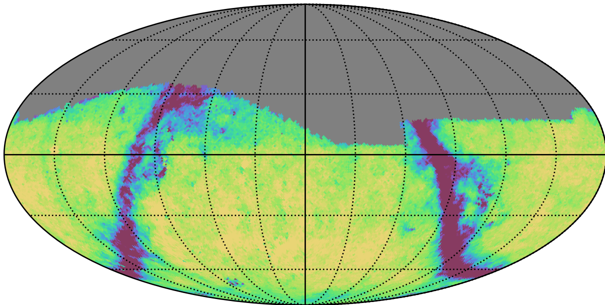
weather_cloudso8v3.4_10yrs Yr 1 g band: Exgal_CoaddM5
