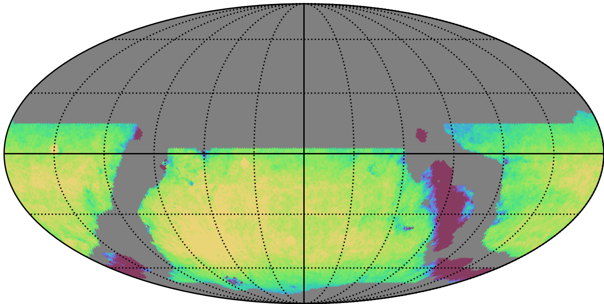
weather_cloudso8v3.4_10yrs WFD z band: Exgal_CoaddM5
