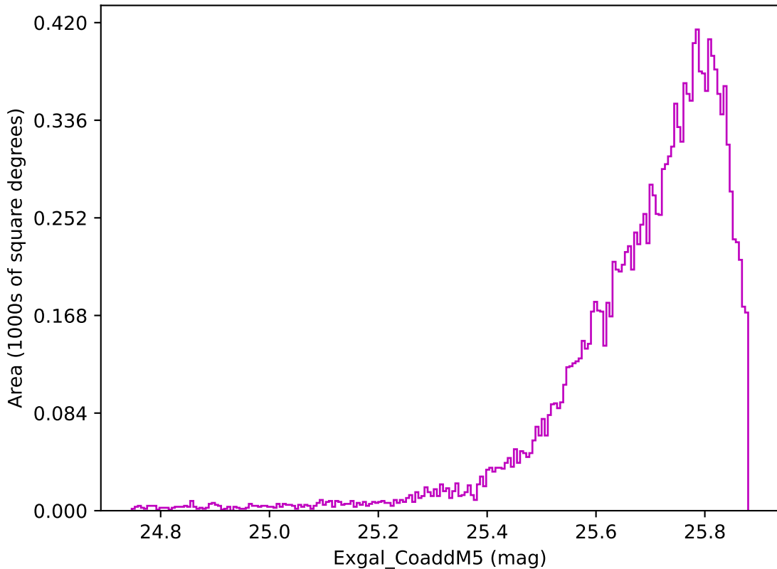
weather_cloudso8v3.4_10yrs WFD z band: Exgal_CoaddM5
