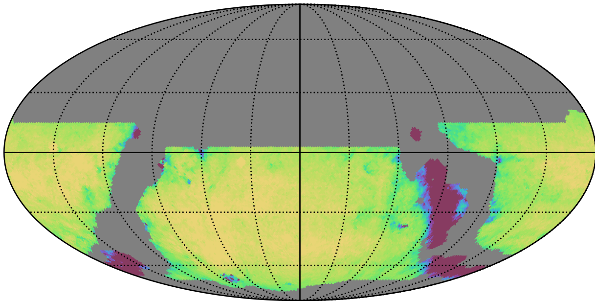
weather_cloudso8v3.4_10yrs WFD u band: Exgal_CoaddM5
