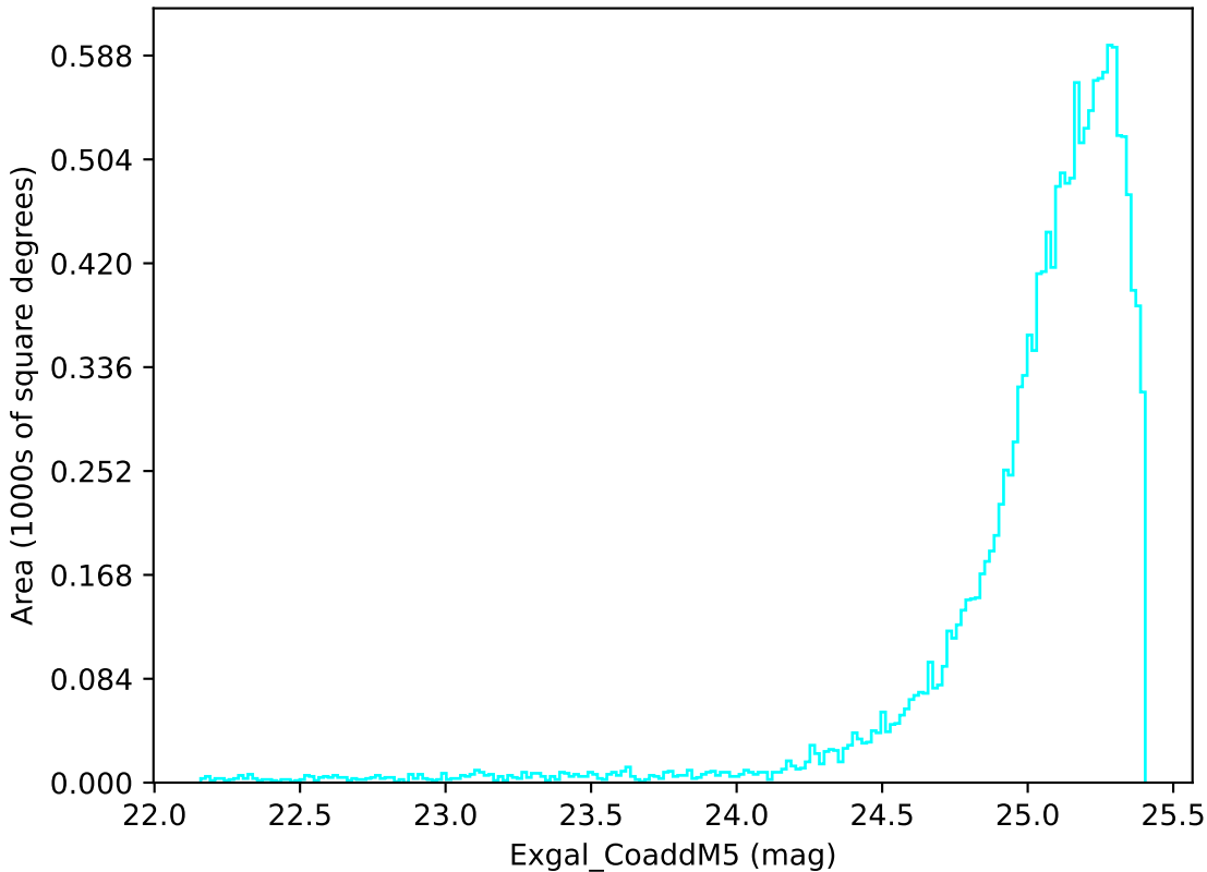
weather_cloudso8v3.4_10yrs WFD u band: Exgal_CoaddM5
