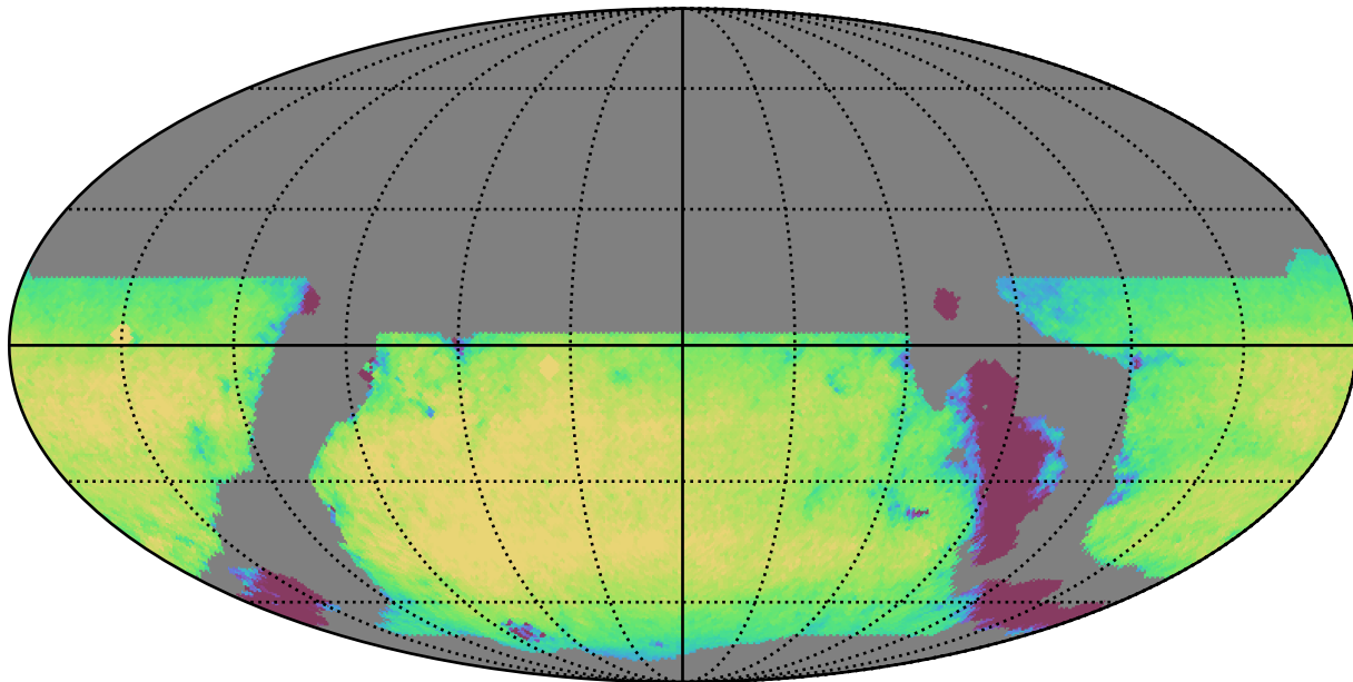
weather_cloudso8v3.4_10yrs WFD i band: Exgal_CoaddM5
